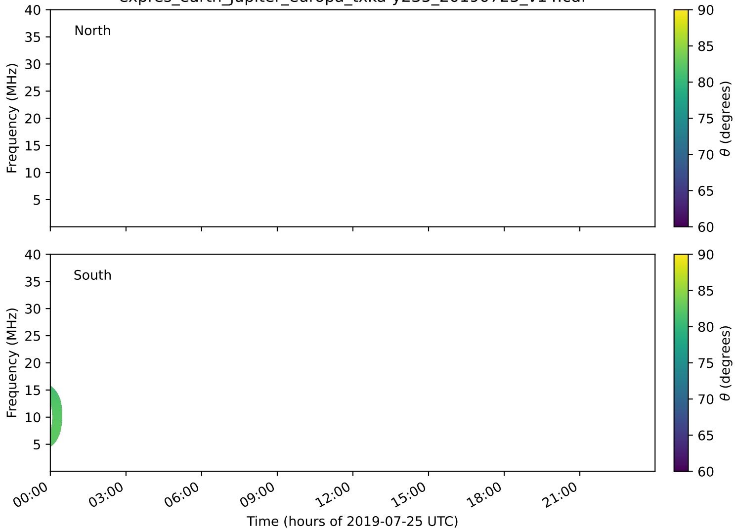
expres_earth_jupiter_europa_txka-y235_20190725_v14.cdf
