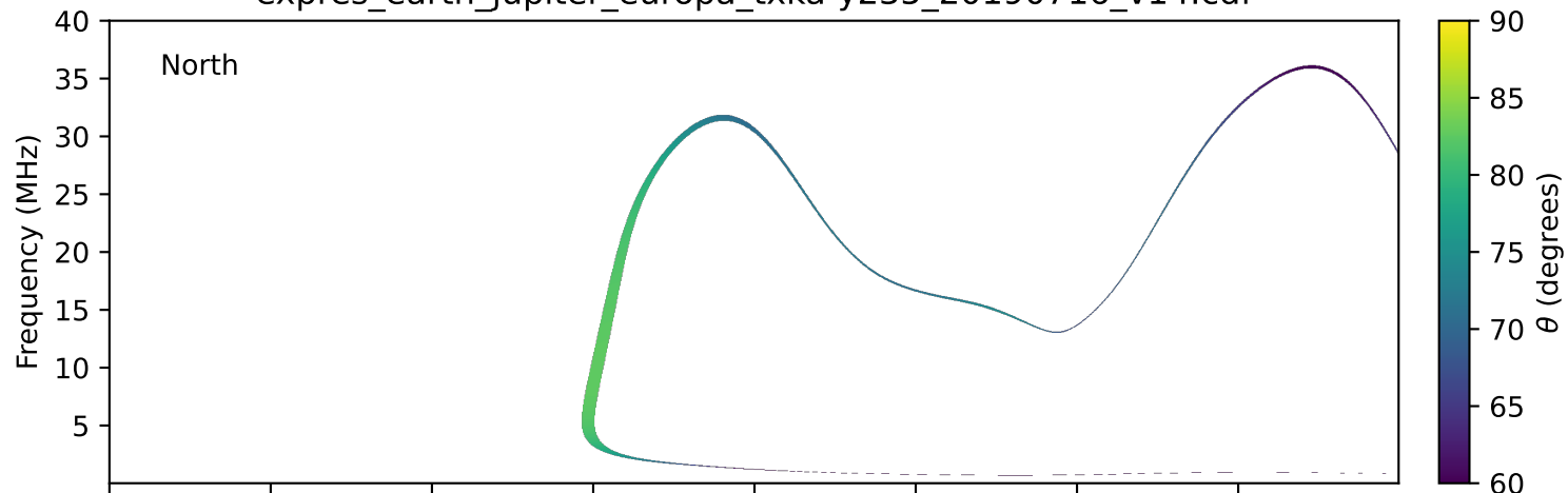
expres_earth_jupiter_europa_txka-y235_20190716_v14.cdf
