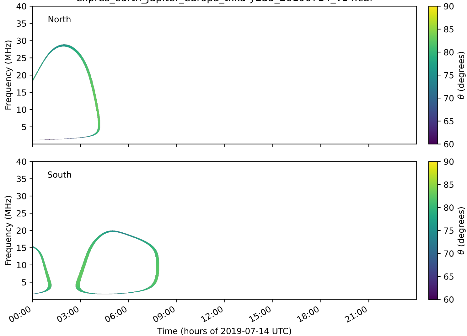
expres_earth_jupiter_europa_txka-y235_20190714_v14.cdf
