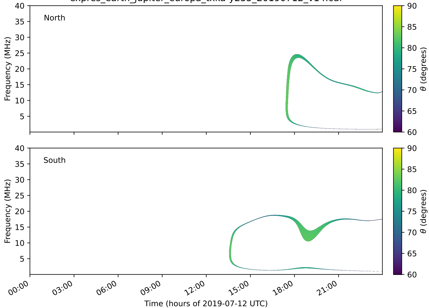
expres_earth_jupiter_europa_txka-y235_20190712_v14.cdf
