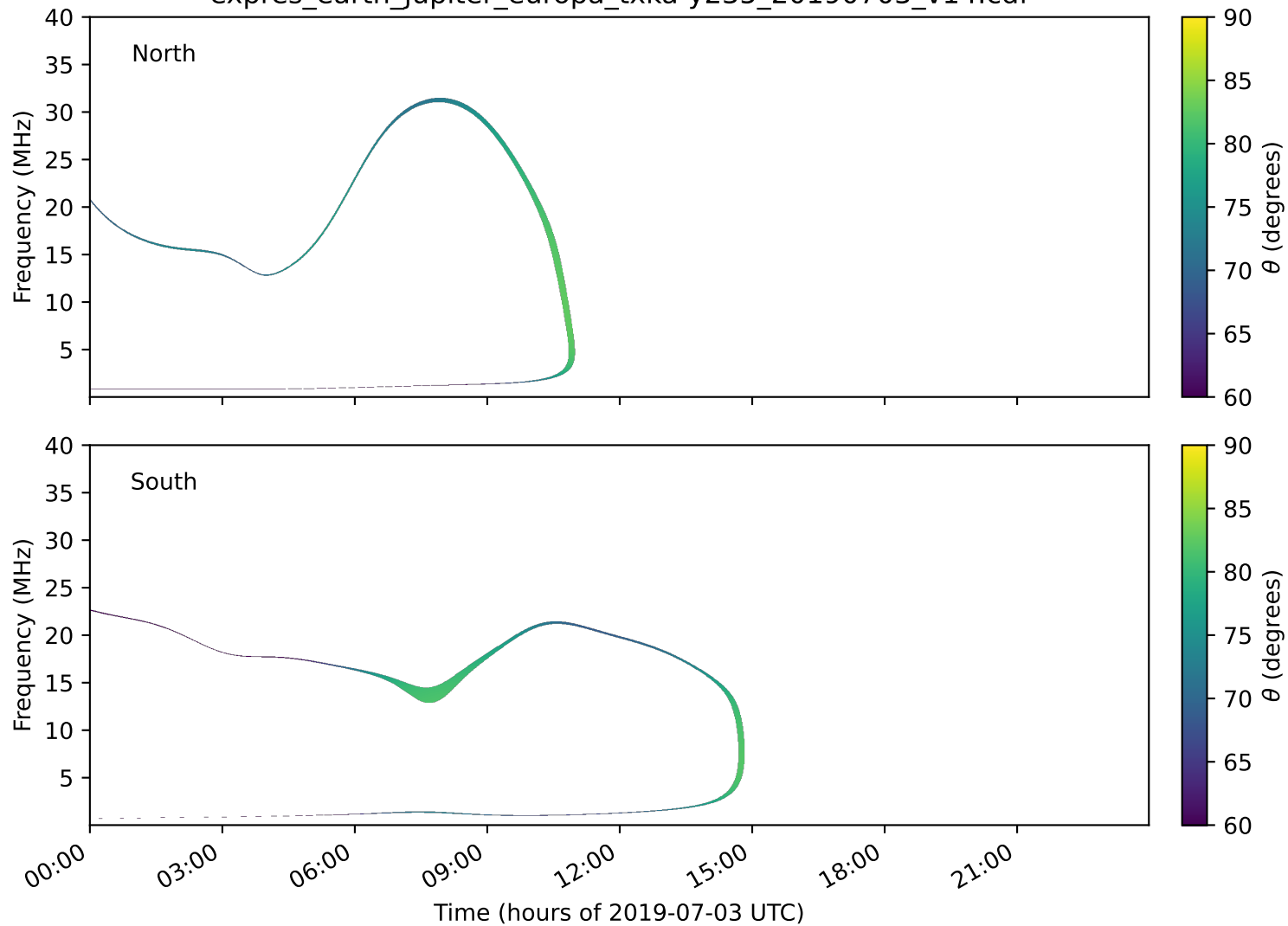
expres_earth_jupiter_europa_txka-y235_20190703_v14.cdf
