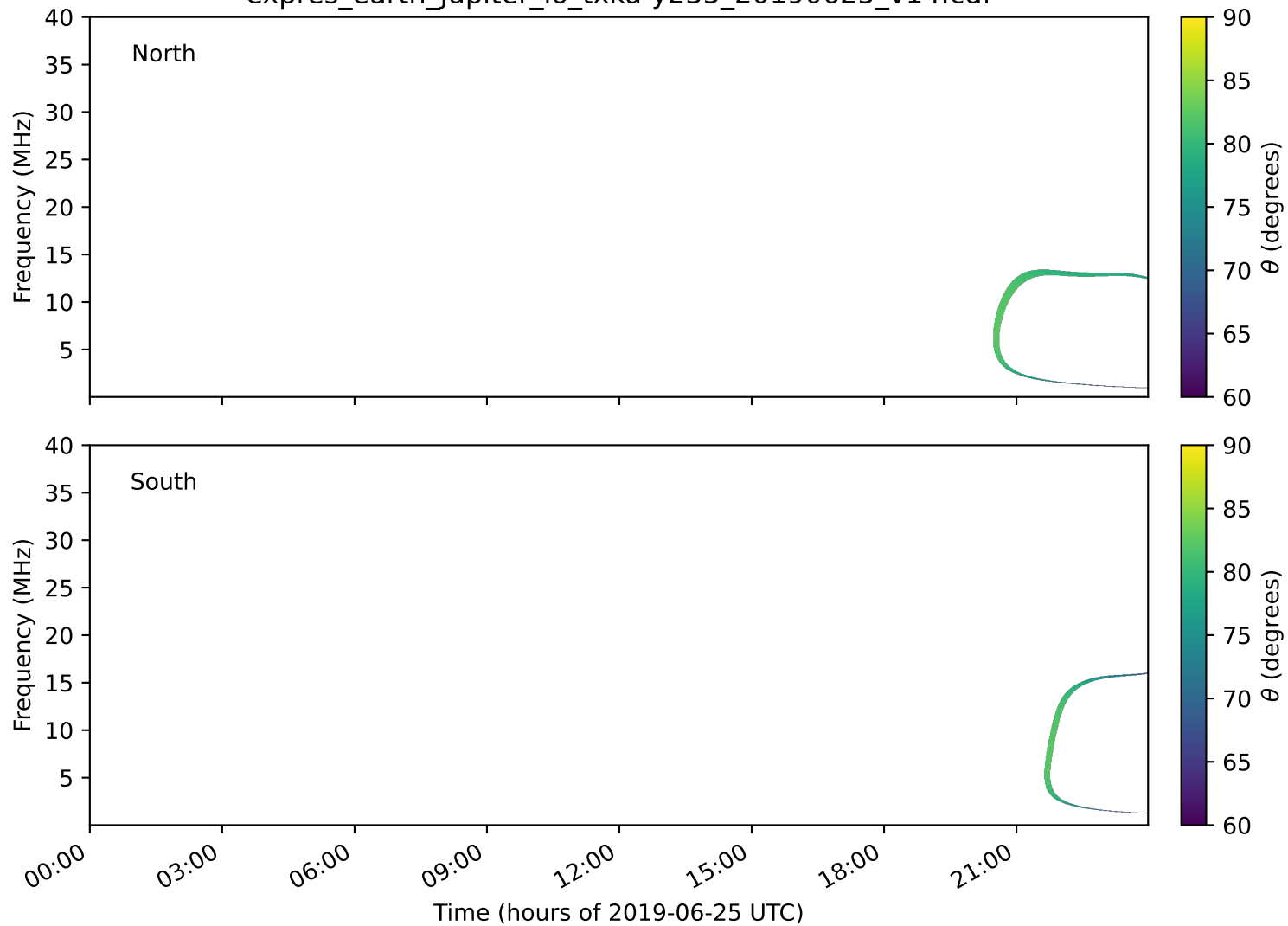
expres_earth_jupiter_io_txka-y235_20190625_v14.cdf
