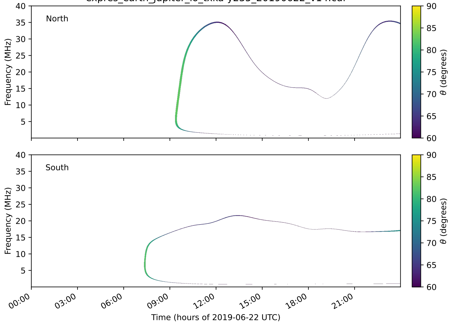
expres_earth_jupiter_io_txka-y235_20190622_v14.cdf
