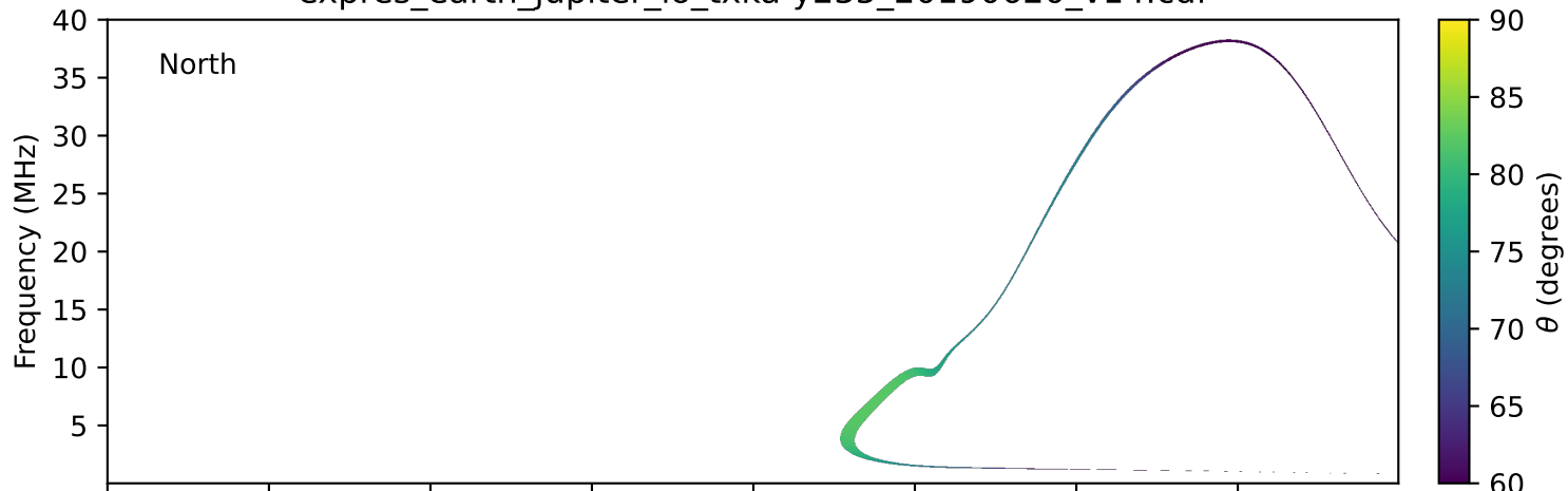
expres_earth_jupiter_io_txka-y235_20190620_v14.cdf
