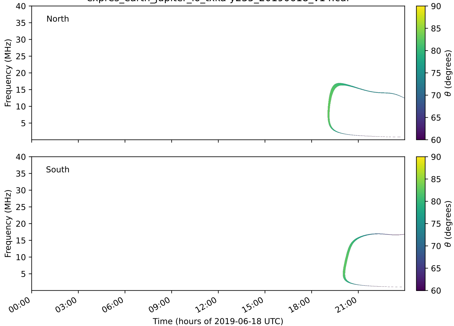
expres_earth_jupiter_io_txka-y235_20190618_v14.cdf
