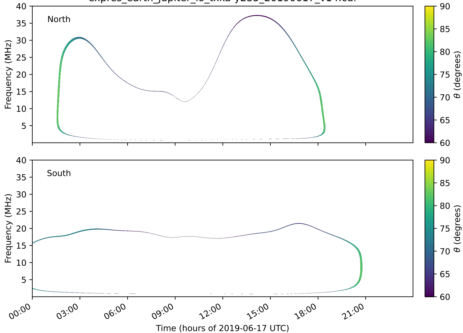
expres_earth_jupiter_io_txka-y235_20190617_v14.cdf
