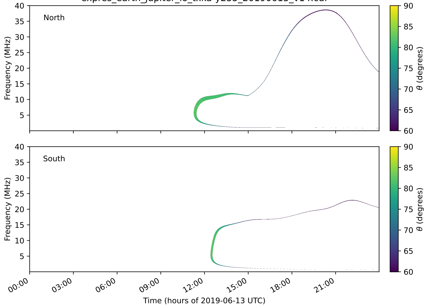
expres_earth_jupiter_io_txka-y235_20190613_v14.cdf
