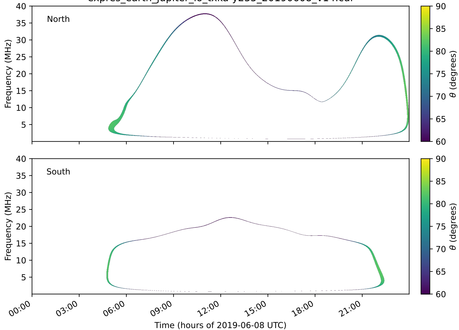
expres_earth_jupiter_io_txka-y235_20190608_v14.cdf
