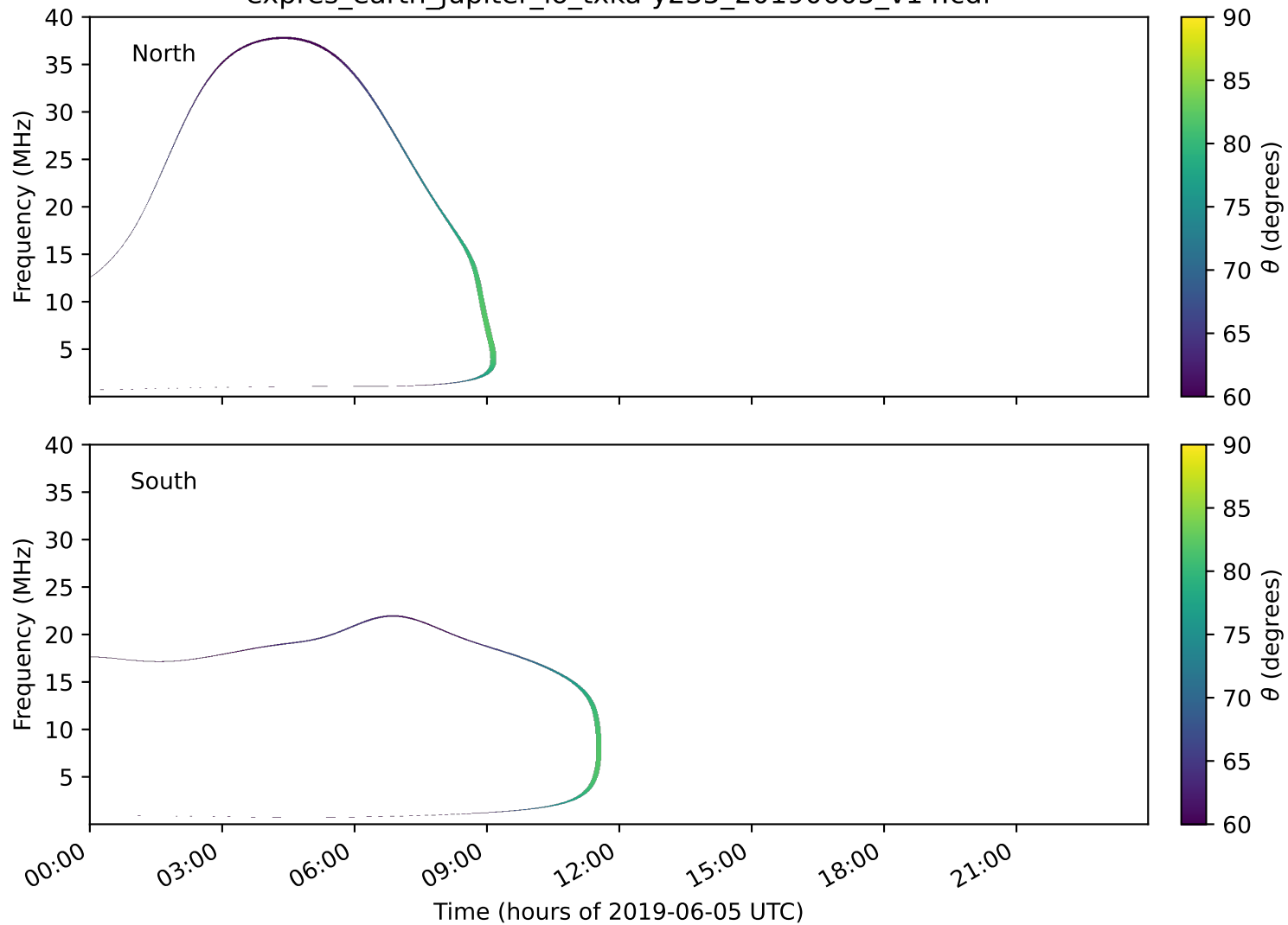
expres_earth_jupiter_io_txka-y235_20190605_v14.cdf
