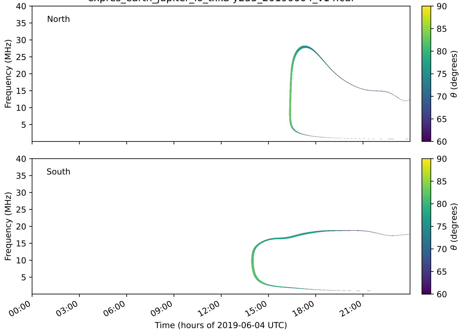
expres_earth_jupiter_io_txka-y235_20190604_v14.cdf
