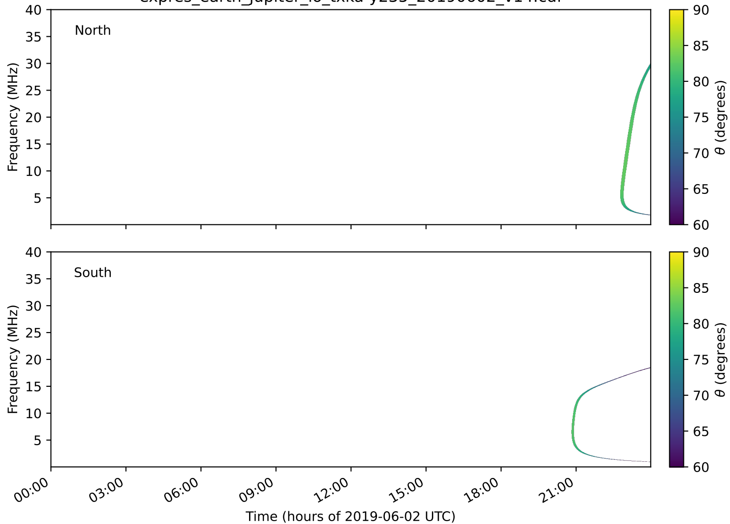
expres_earth_jupiter_io_txka-y235_20190602_v14.cdf
