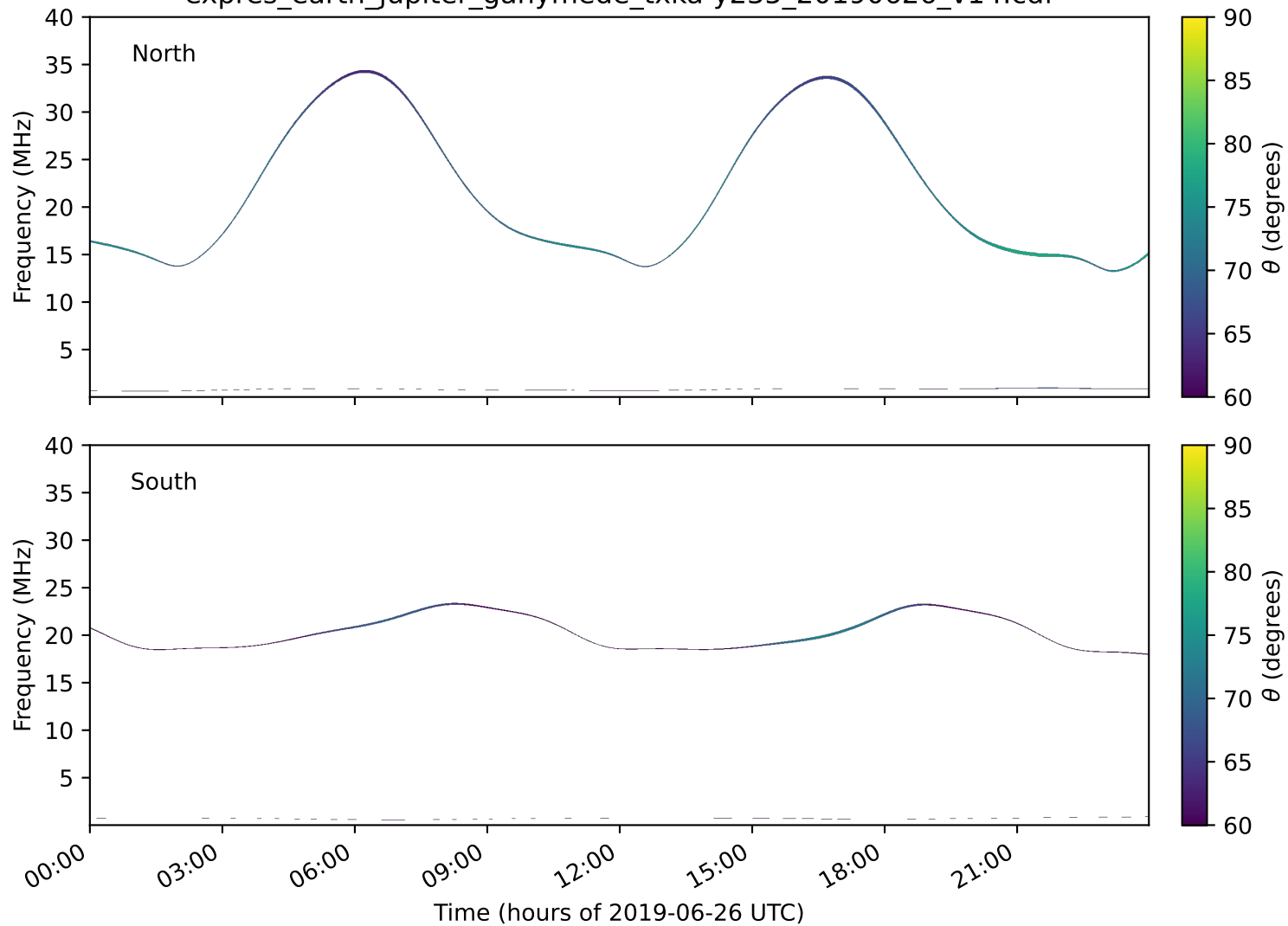
expres_earth_jupiter_ganymede_txka-y235_20190626_v14.cdf
