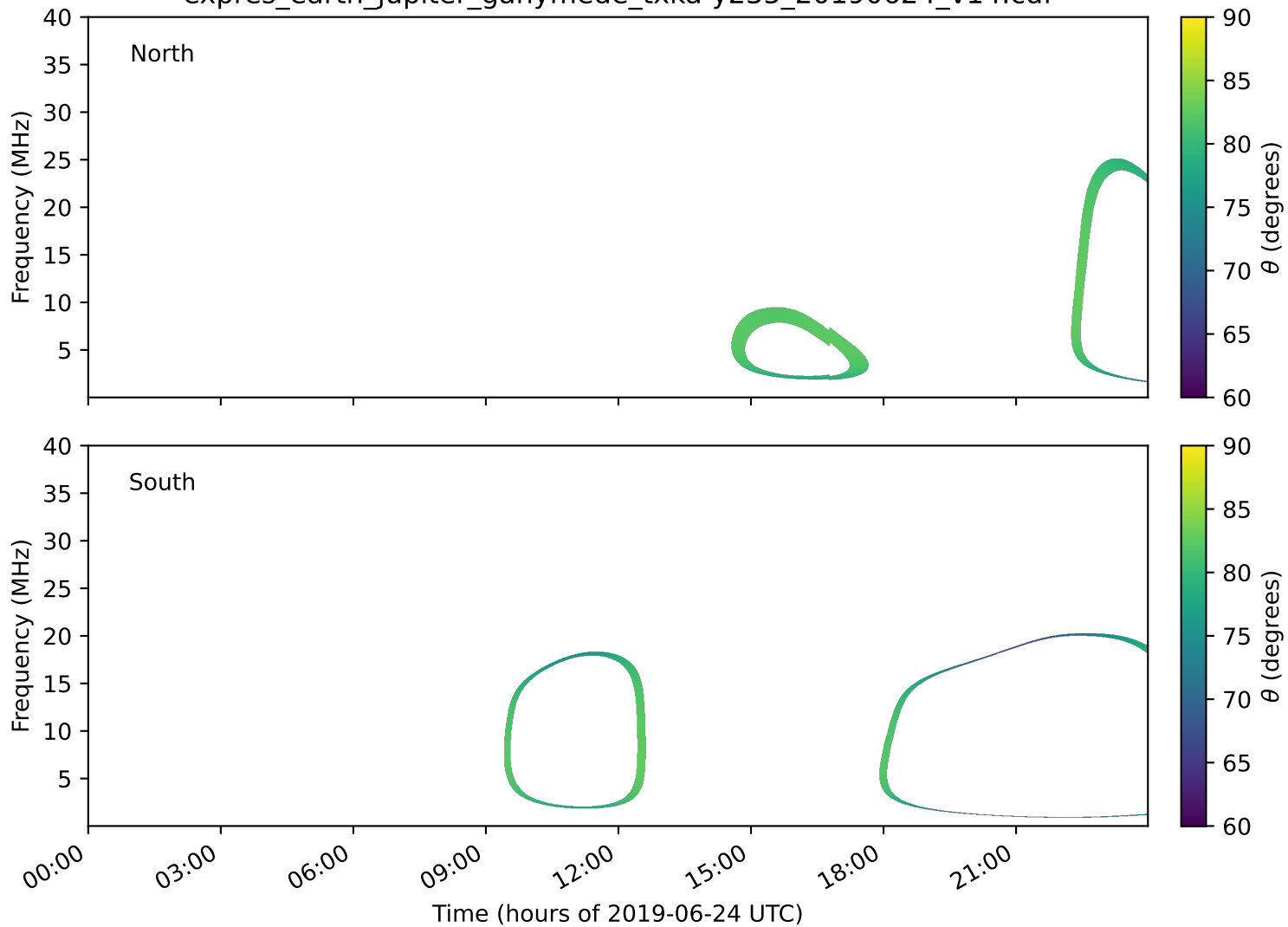
expres_earth_jupiter_ganymede_txka-y235_20190624_v14.cdf
