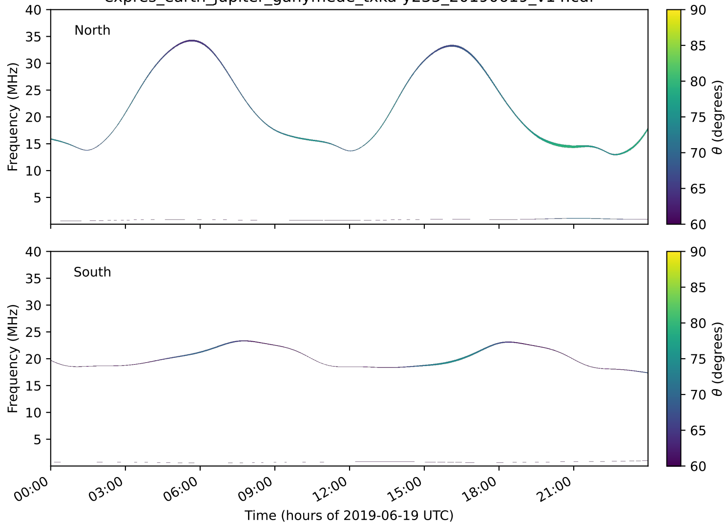
expres_earth_jupiter_ganymede_txka-y235_20190619_v14.cdf
