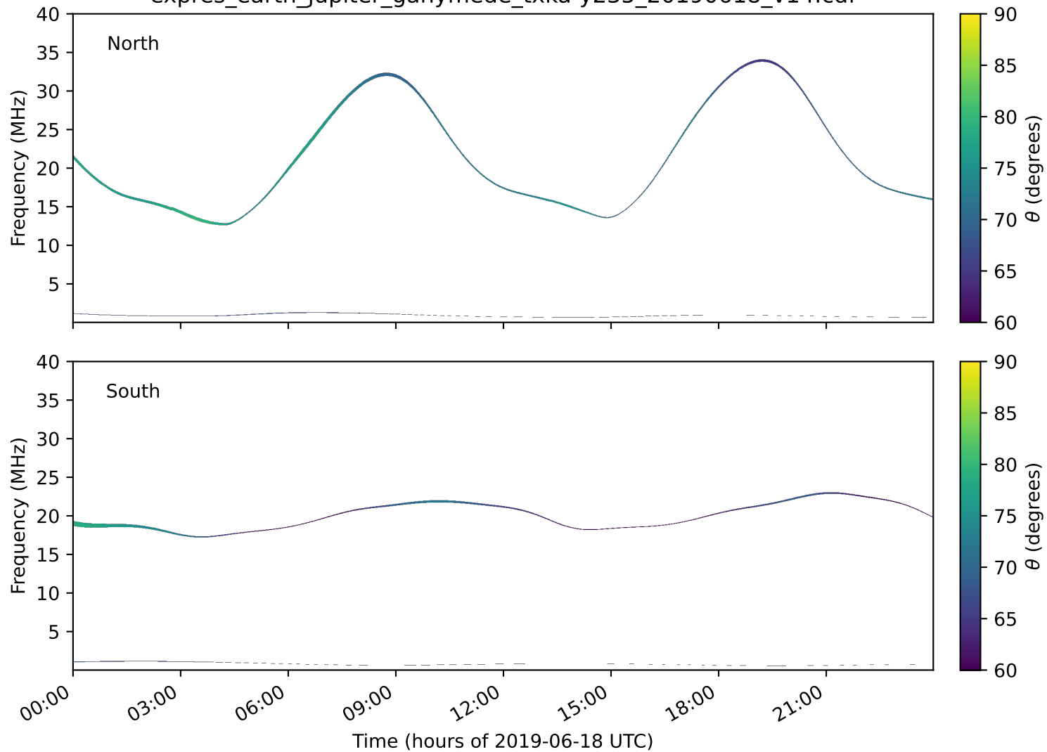
expres_earth_jupiter_ganymede_txka-y235_20190618_v14.cdf
