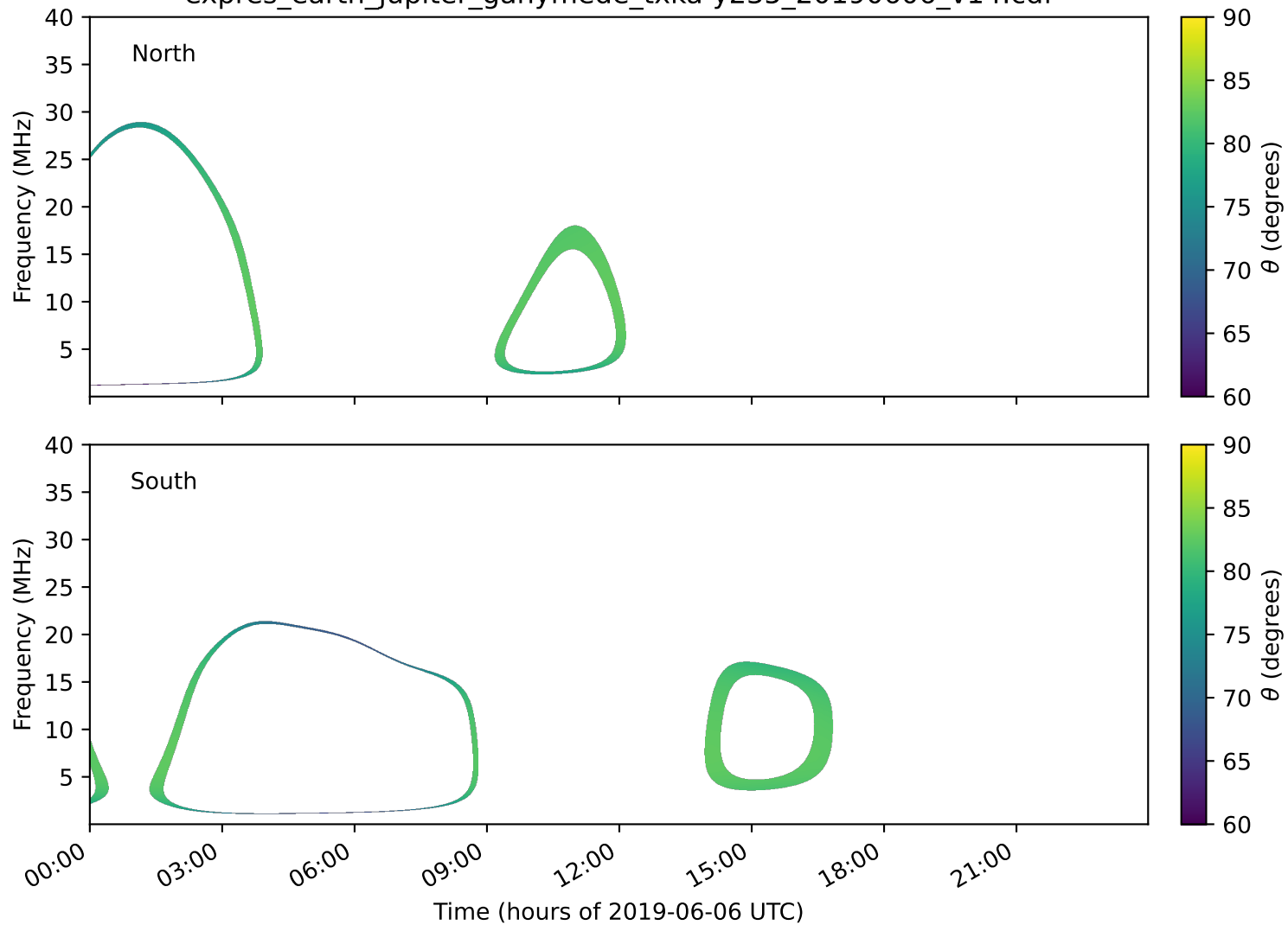
expres_earth_jupiter_ganymede_txka-y235_20190606_v14.cdf
