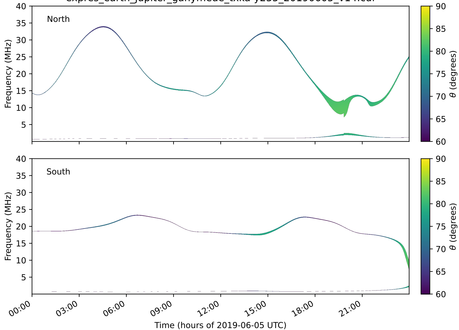
expres_earth_jupiter_ganymede_txka-y235_20190605_v14.cdf
