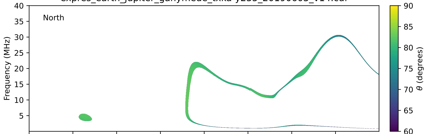
expres_earth_jupiter_ganymede_txka-y235_20190603_v14.cdf
