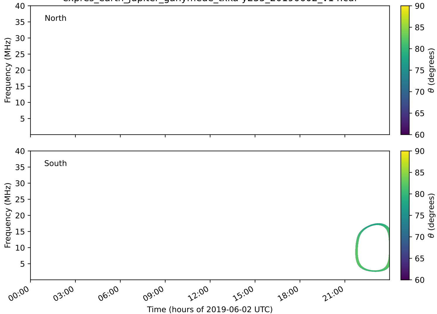
expres_earth_jupiter_ganymede_txka-y235_20190602_v14.cdf
