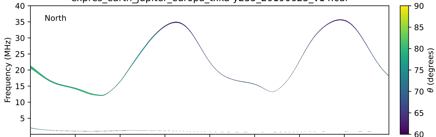
expres_earth_jupiter_europa_txka-y235_20190625_v14.cdf
