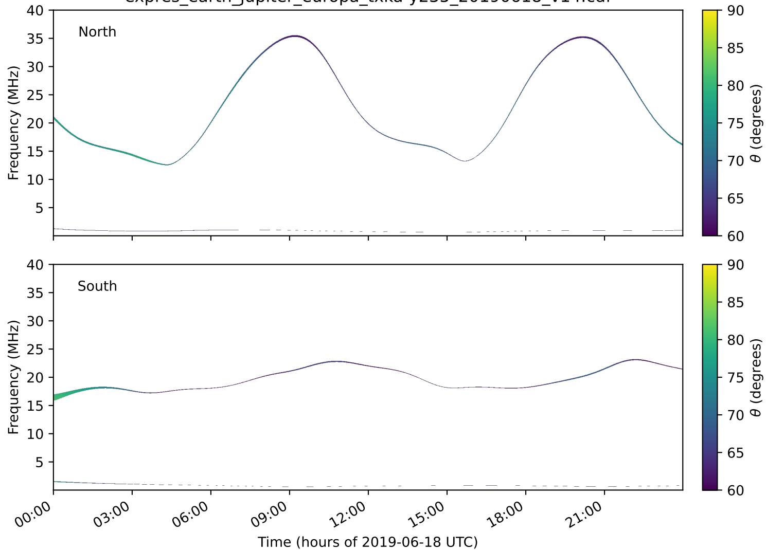
expres_earth_jupiter_europa_txka-y235_20190618_v14.cdf
