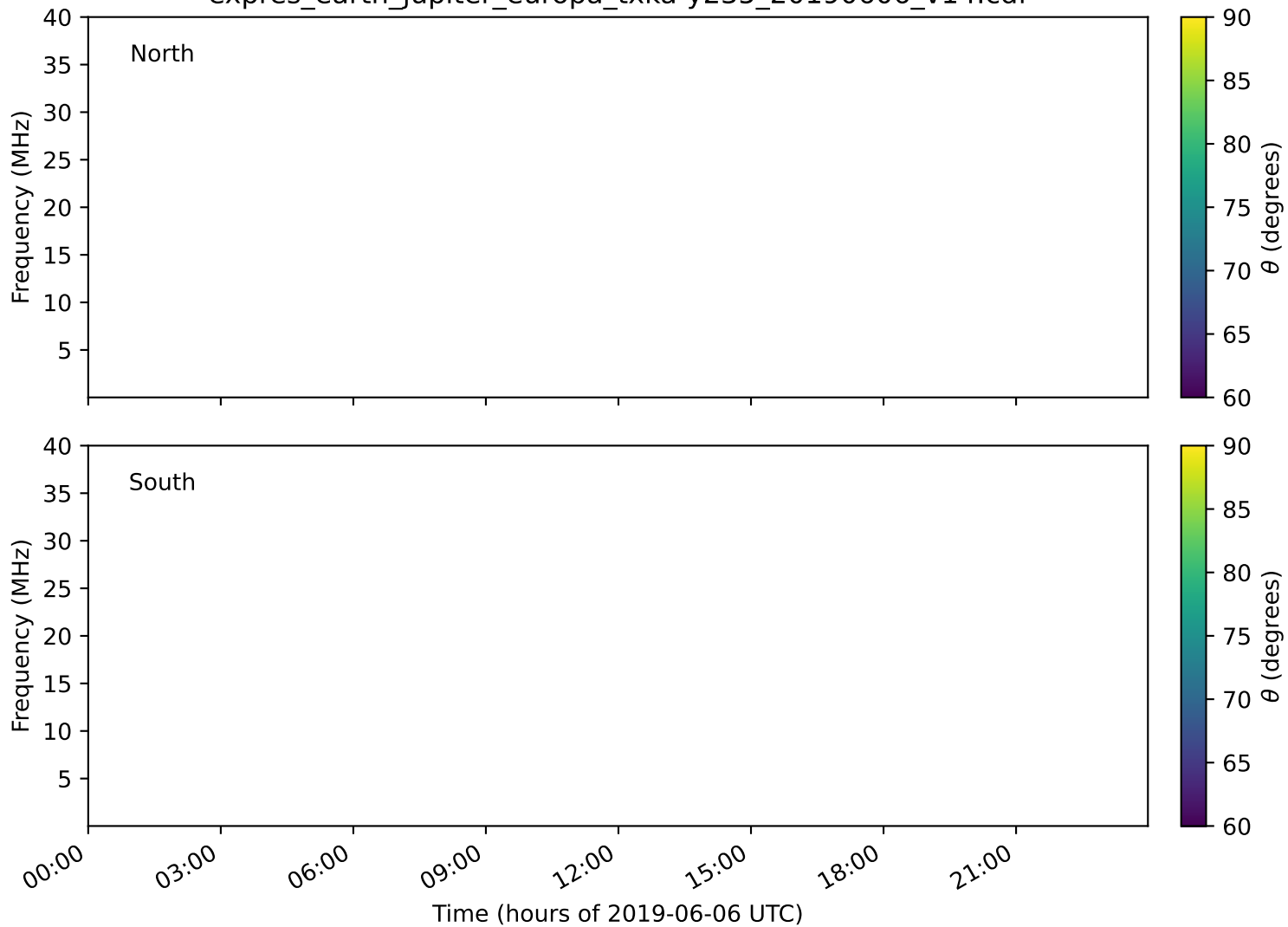
expres_earth_jupiter_europa_txka-y235_20190606_v14.cdf
