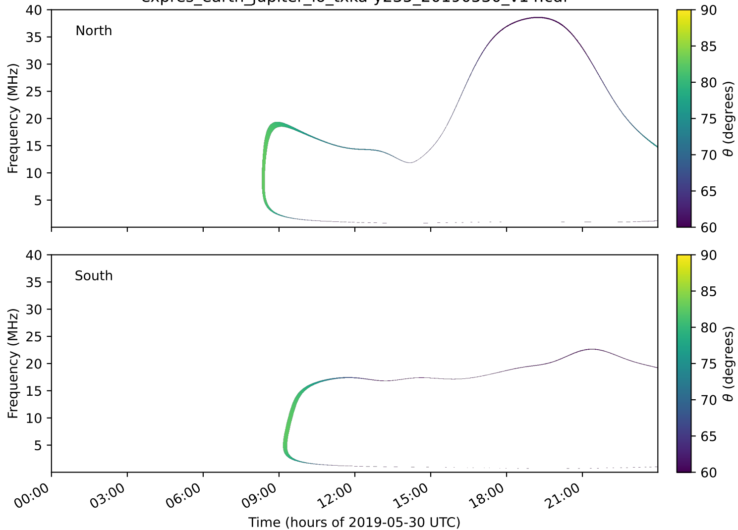
expres_earth_jupiter_io_txka-y235_20190530_v14.cdf
