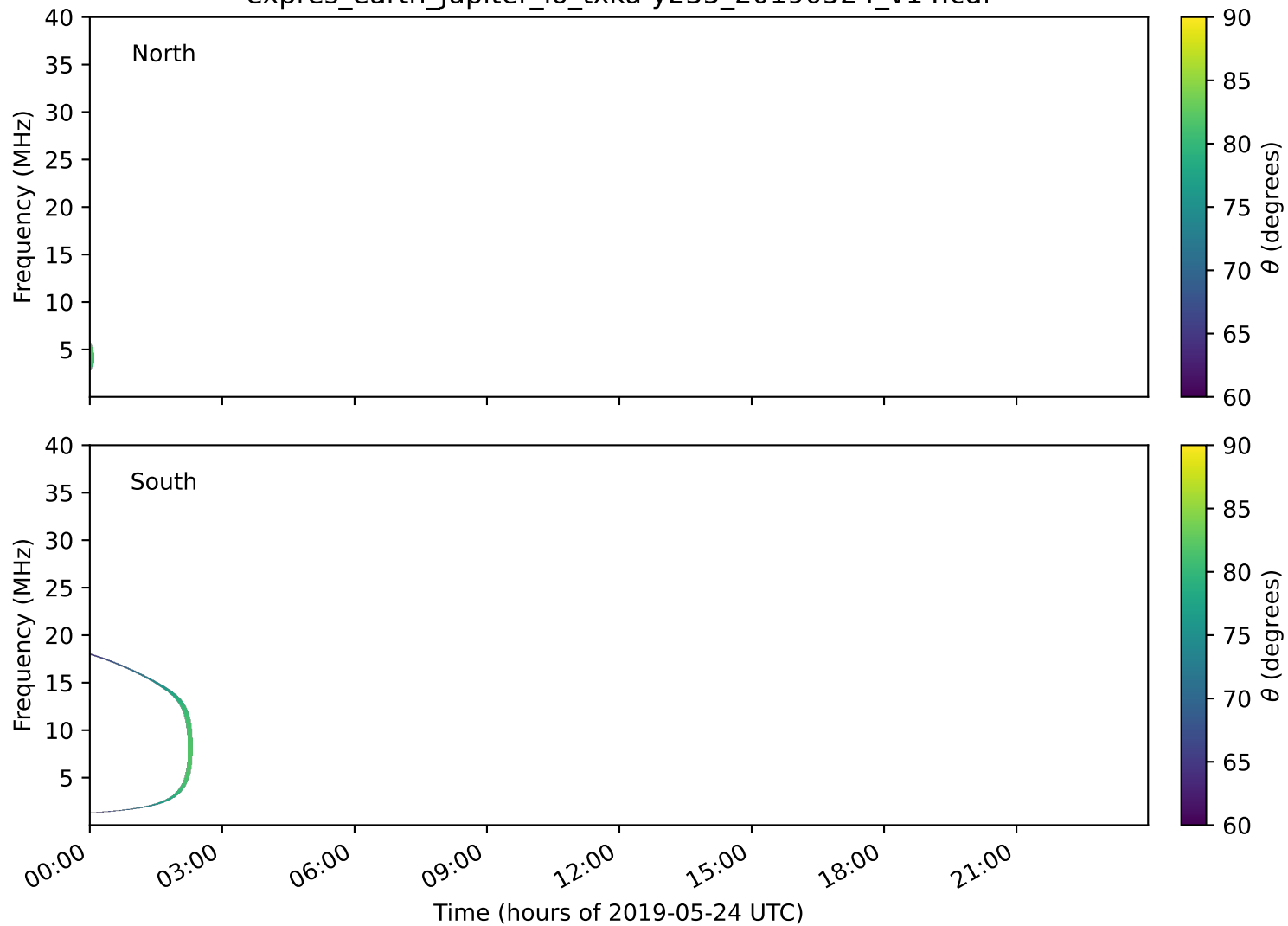
expres_earth_jupiter_io_txka-y235_20190524_v14.cdf
