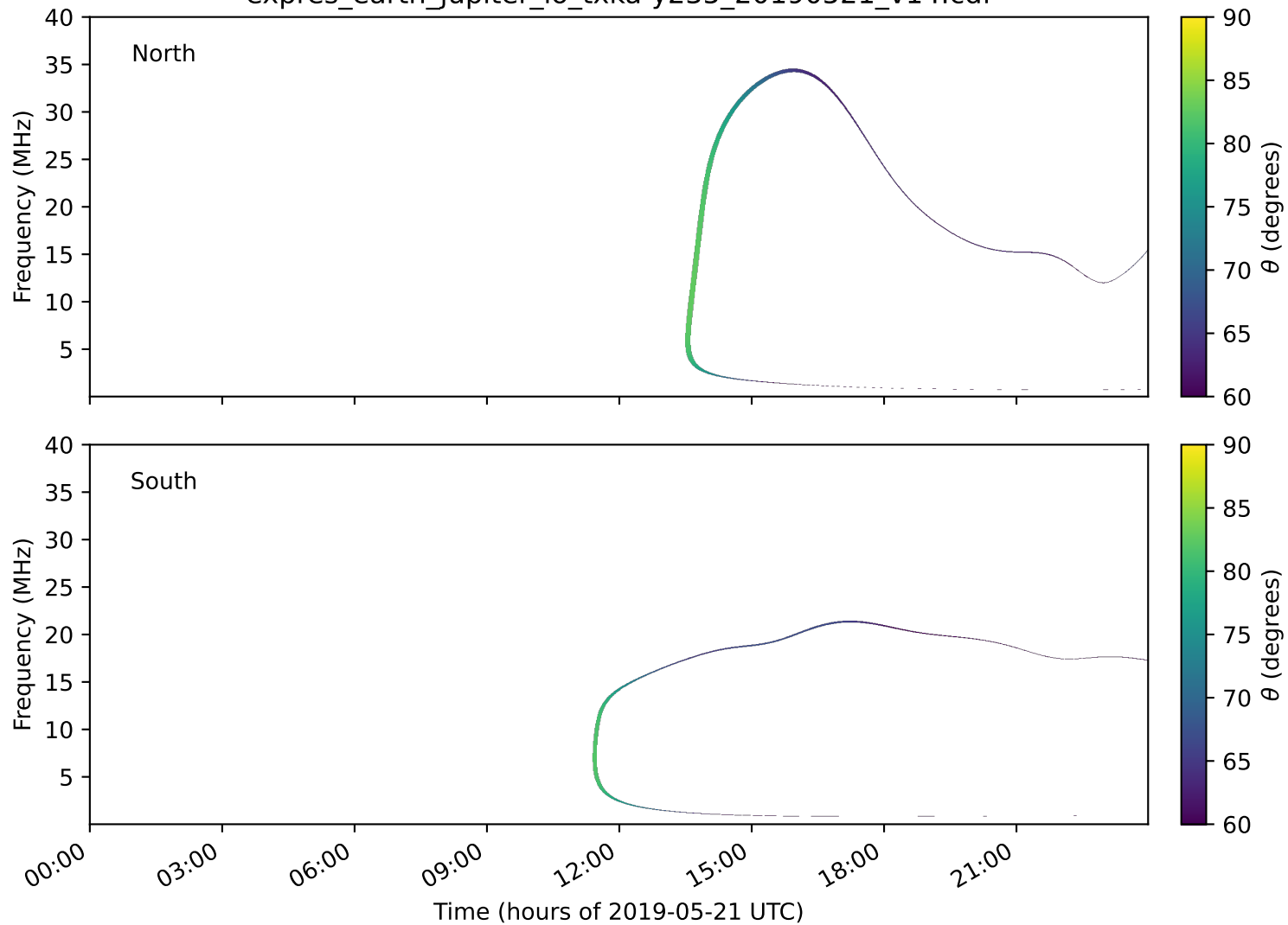
expres_earth_jupiter_io_txka-y235_20190521_v14.cdf
