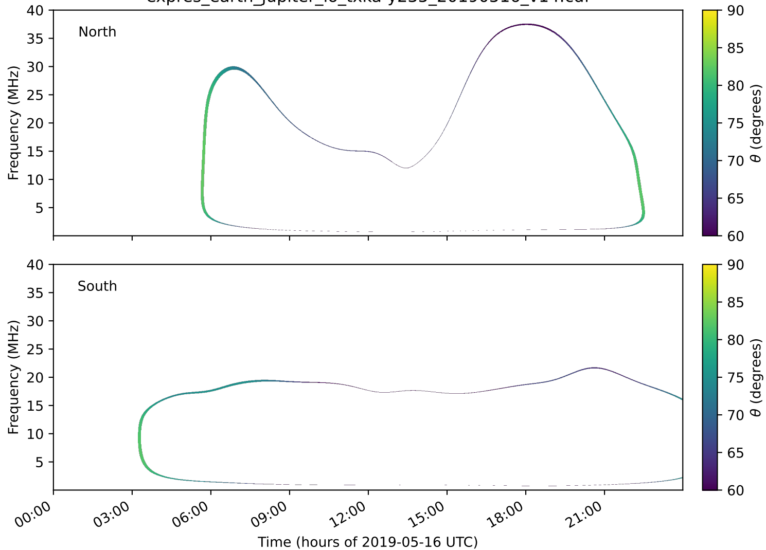
expres_earth_jupiter_io_txka-y235_20190516_v14.cdf
