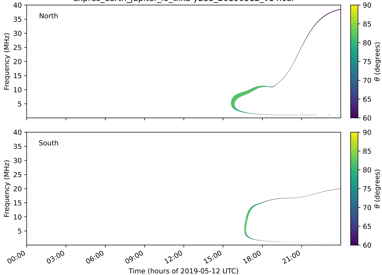
expres_earth_jupiter_io_txka-y235_20190512_v14.cdf
