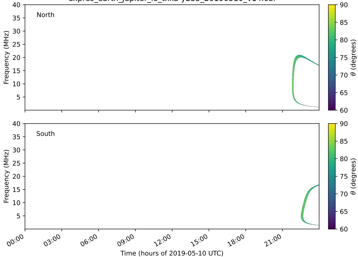
expres_earth_jupiter_io_txka-y235_20190510_v14.cdf
