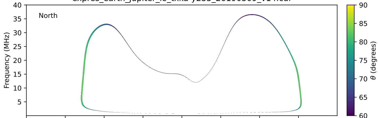
expres_earth_jupiter_io_txka-y235_20190509_v14.cdf
