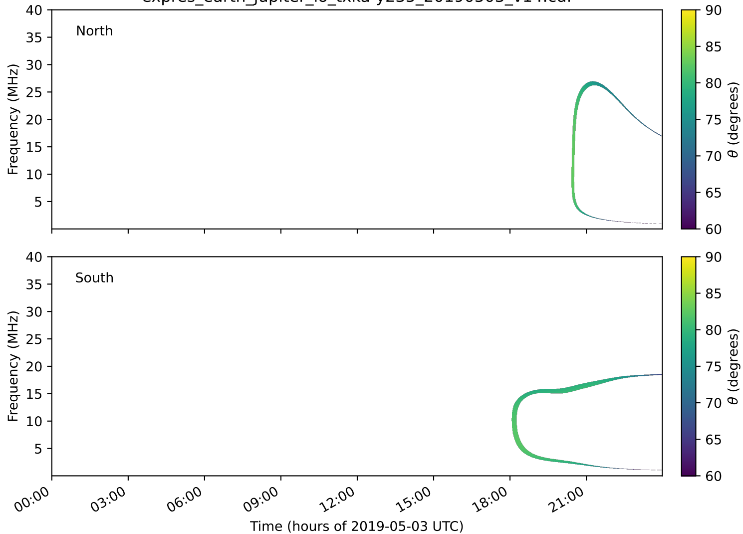
expres_earth_jupiter_io_txka-y235_20190503_v14.cdf
