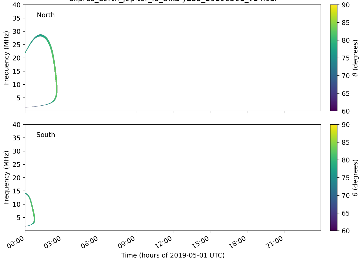
expres_earth_jupiter_io_txka-y235_20190501_v14.cdf
