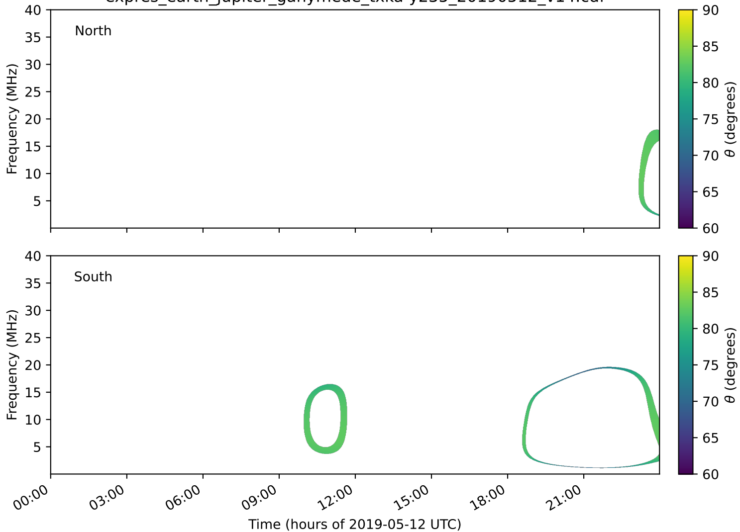
expres_earth_jupiter_ganymede_txka-y235_20190512_v14.cdf
