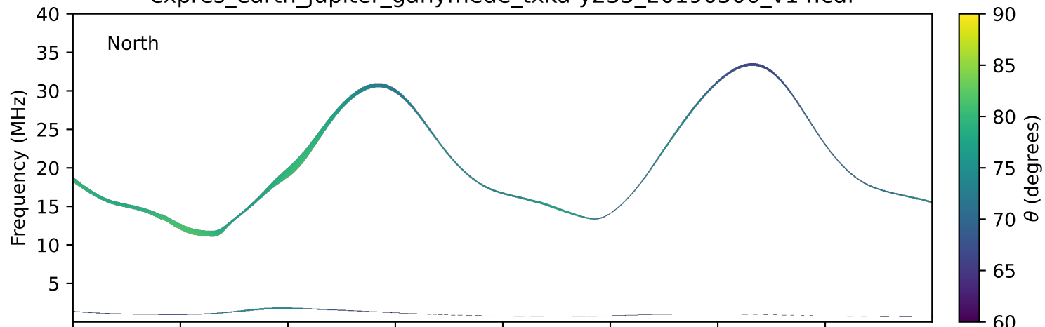
expres_earth_jupiter_ganymede_txka-y235_20190506_v14.cdf
