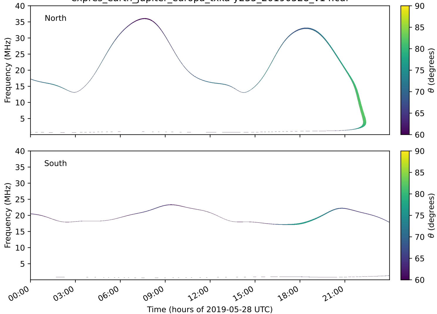
expres_earth_jupiter_europa_txka-y235_20190528_v14.cdf
