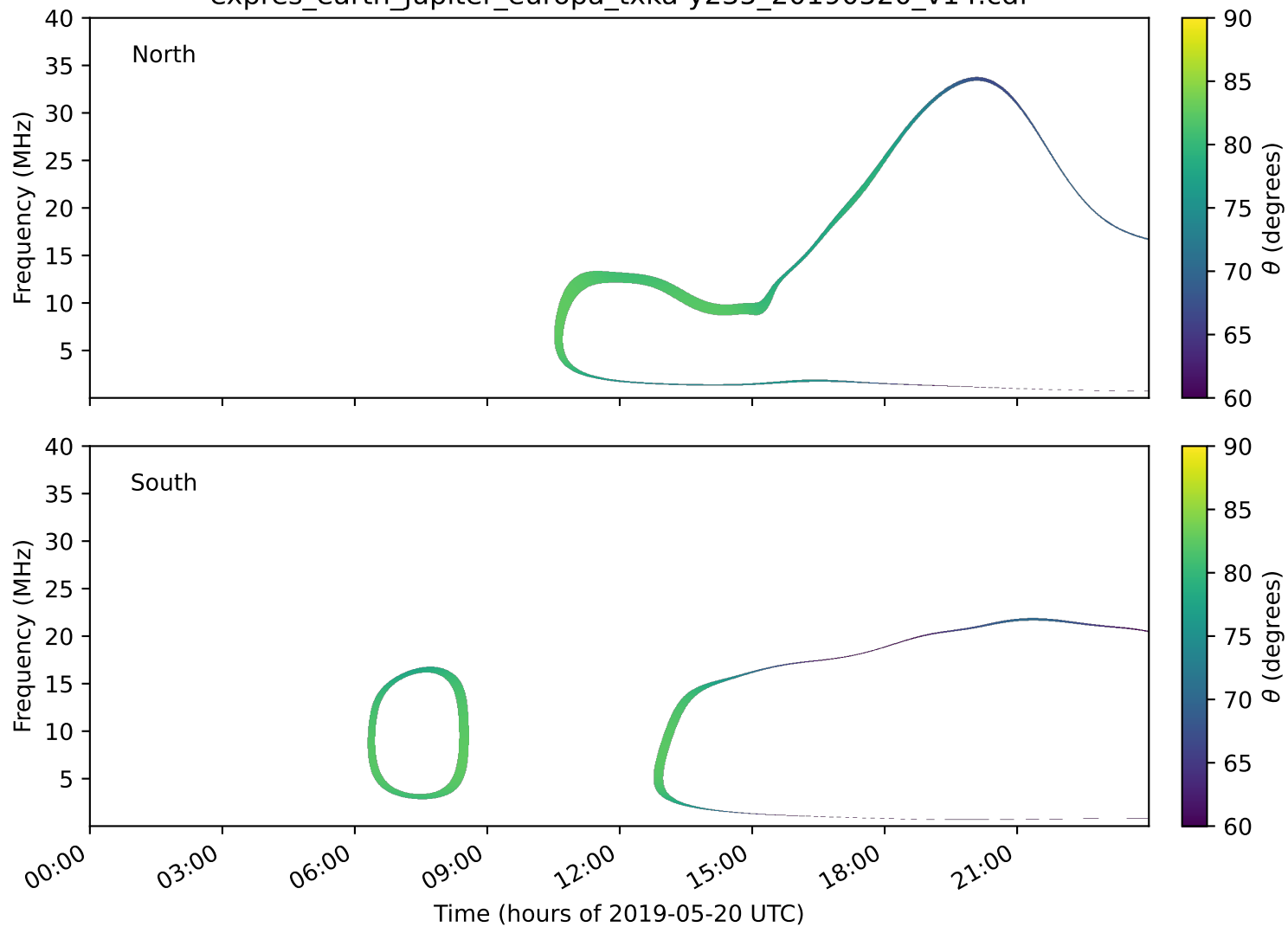
expres_earth_jupiter_europa_txka-y235_20190520_v14.cdf
