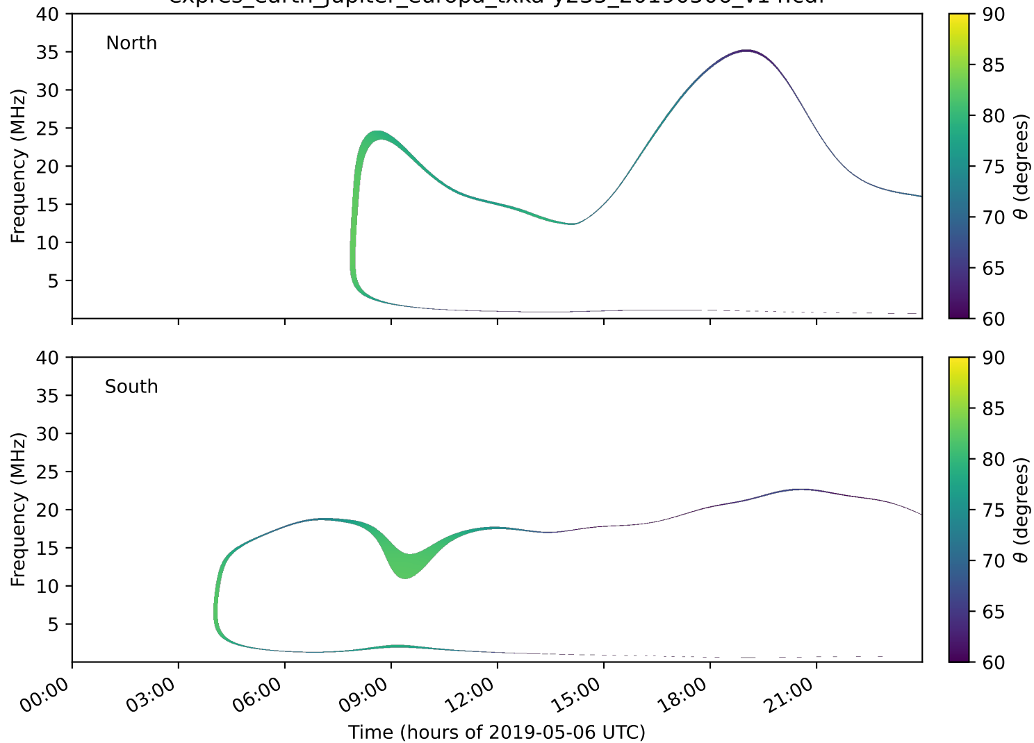
expres_earth_jupiter_europa_txka-y235_20190506_v14.cdf
