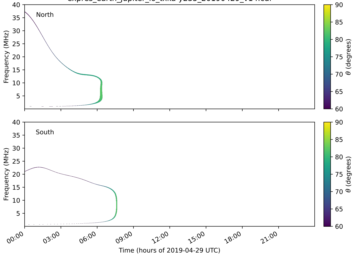
expres_earth_jupiter_io_txka-y235_20190429_v14.cdf
