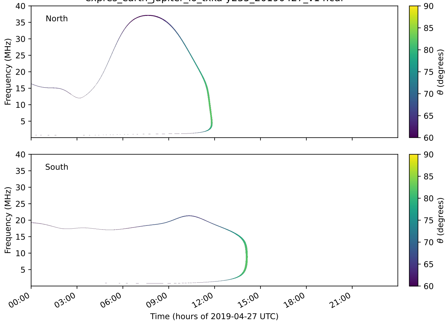
expres_earth_jupiter_io_txka-y235_20190427_v14.cdf
