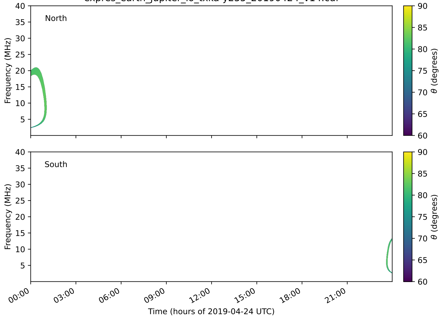
expres_earth_jupiter_io_txka-y235_20190424_v14.cdf
