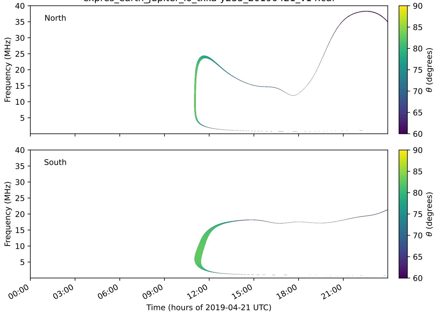
expres_earth_jupiter_io_txka-y235_20190421_v14.cdf
