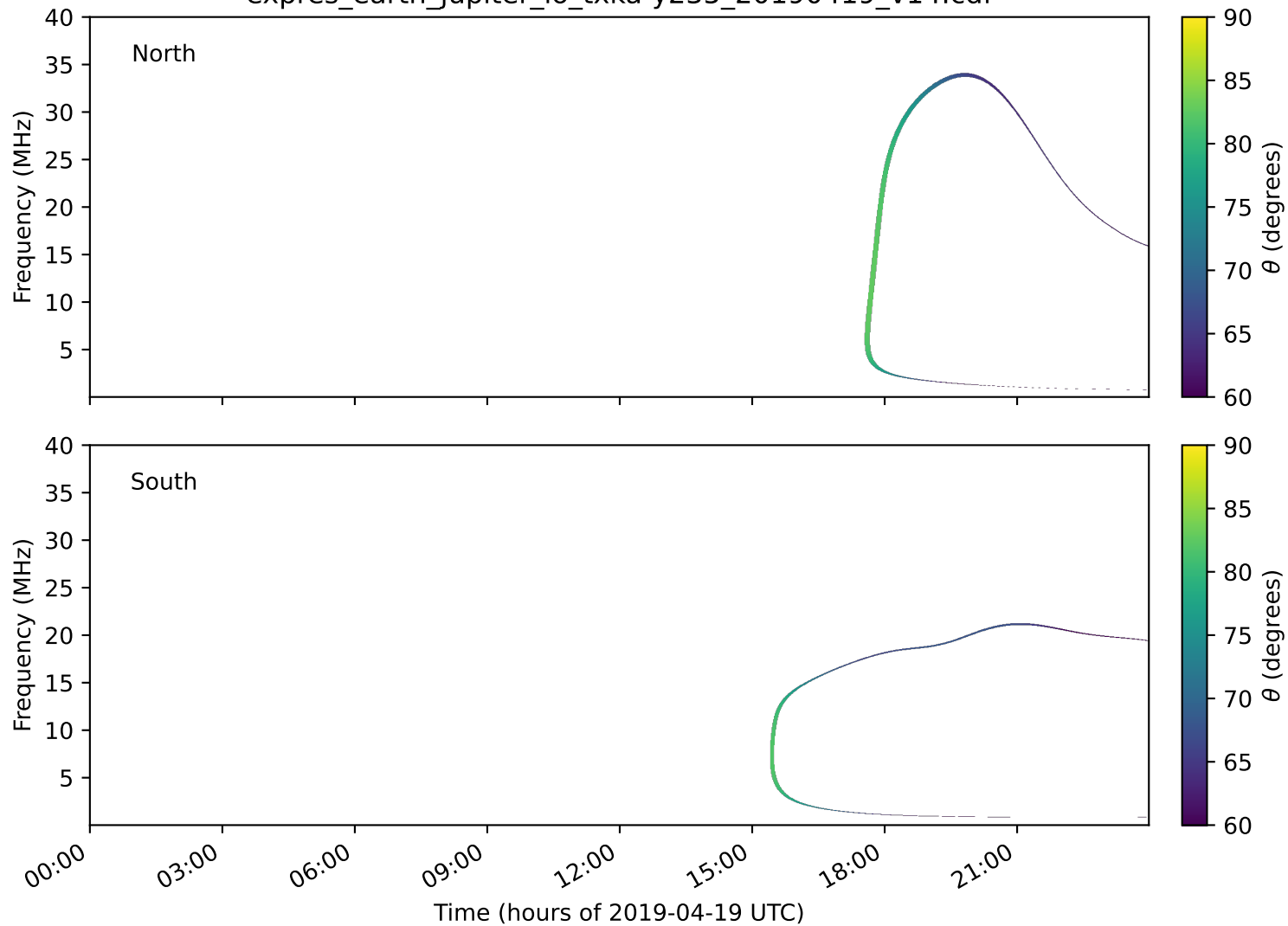
expres_earth_jupiter_io_txka-y235_20190419_v14.cdf
