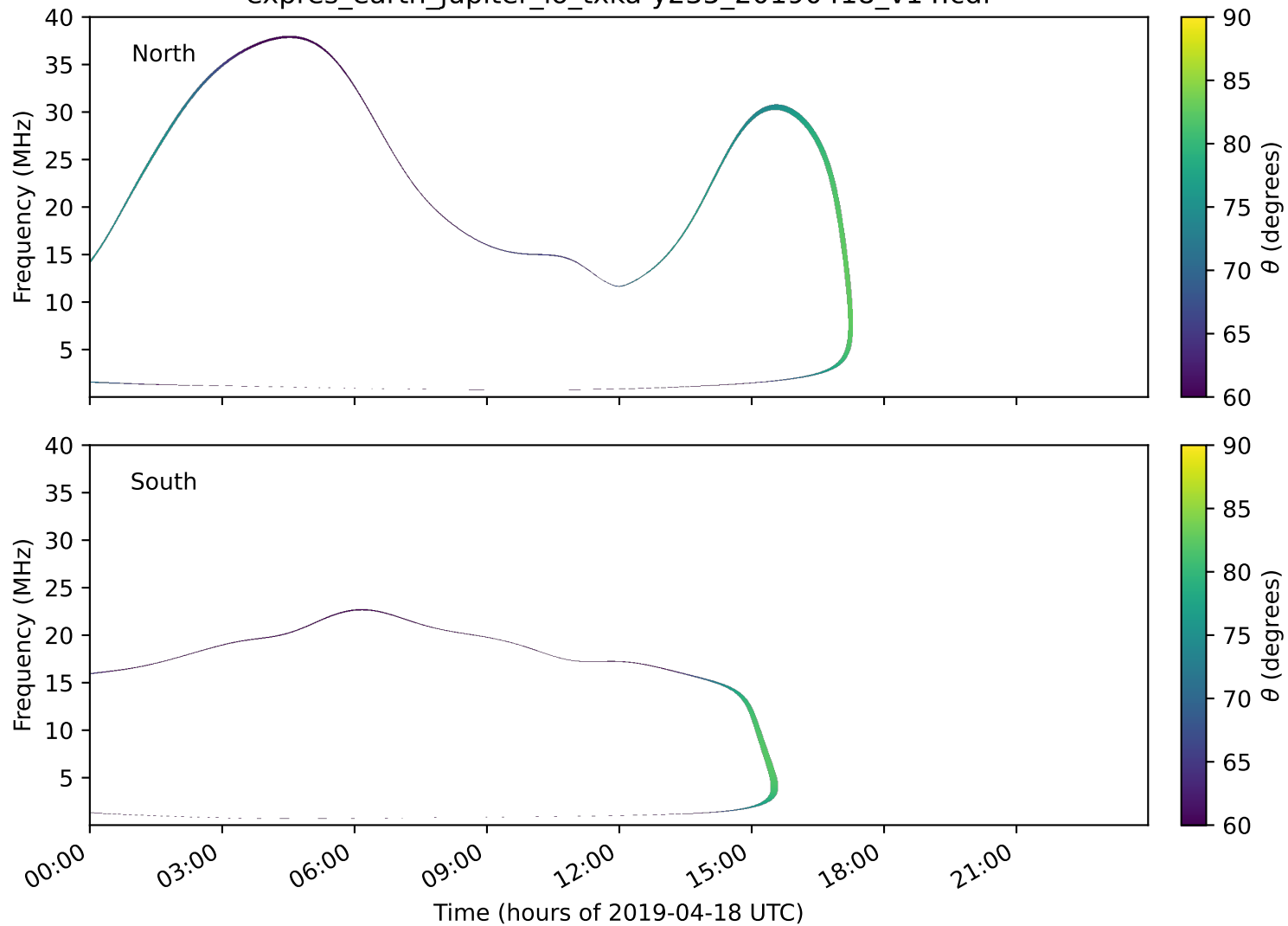
expres_earth_jupiter_io_txka-y235_20190418_v14.cdf
