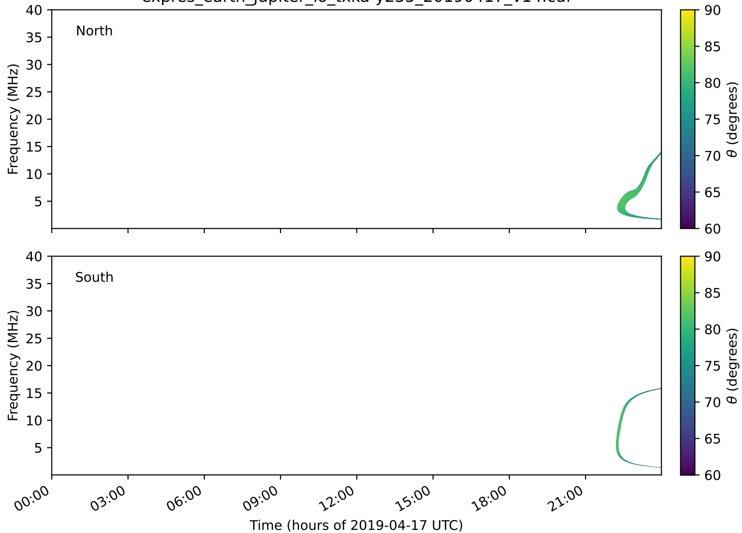
expres_earth_jupiter_io_txka-y235_20190417_v14.cdf
