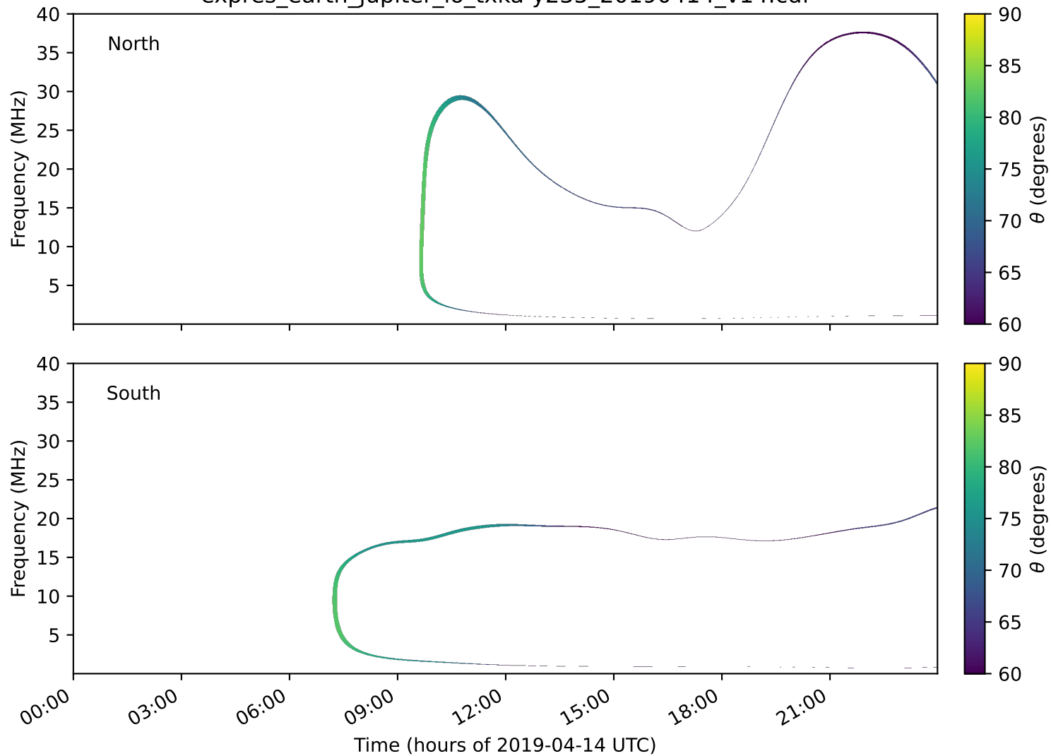
expres_earth_jupiter_io_txka-y235_20190414_v14.cdf
