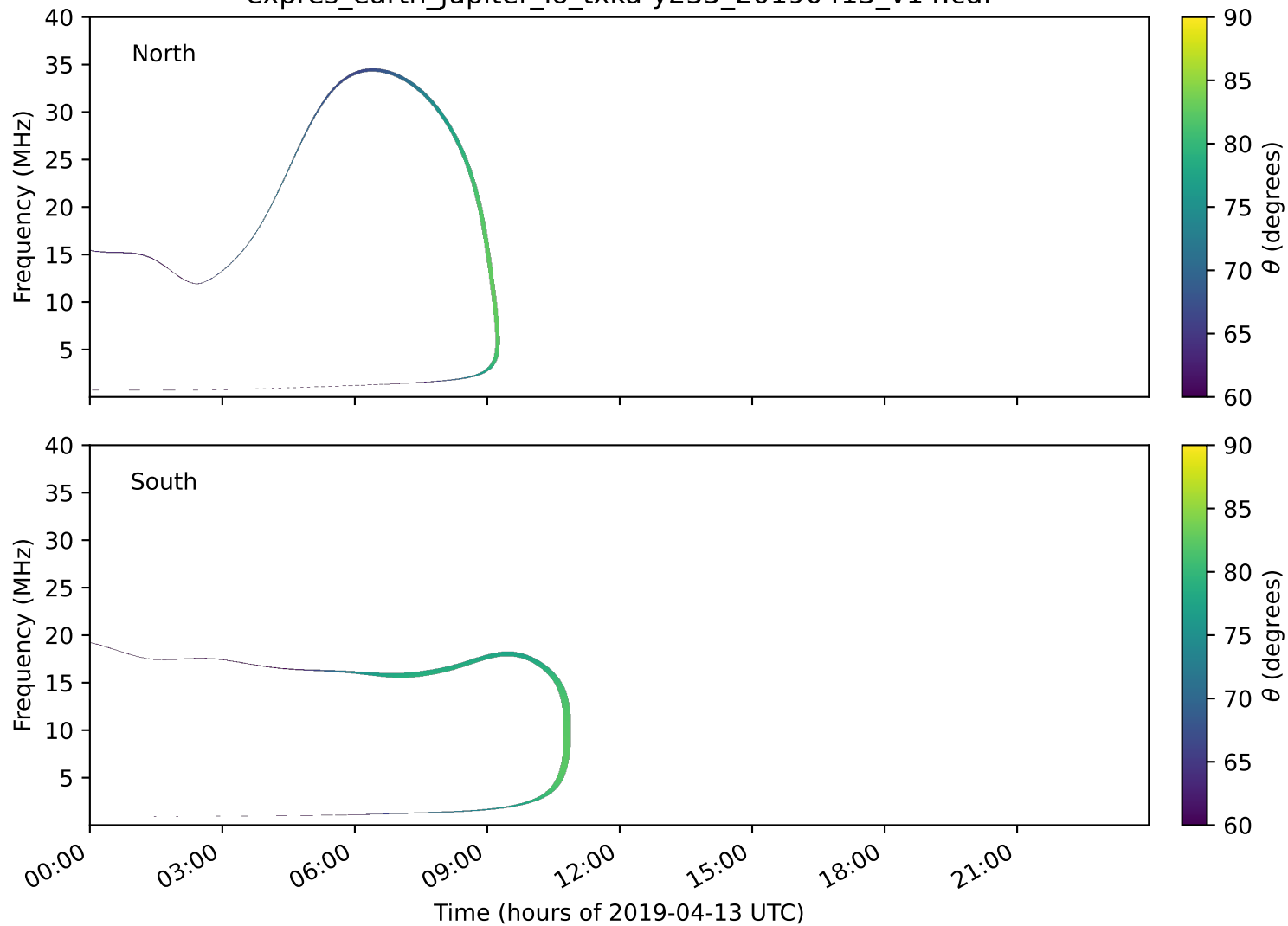
expres_earth_jupiter_io_txka-y235_20190413_v14.cdf
