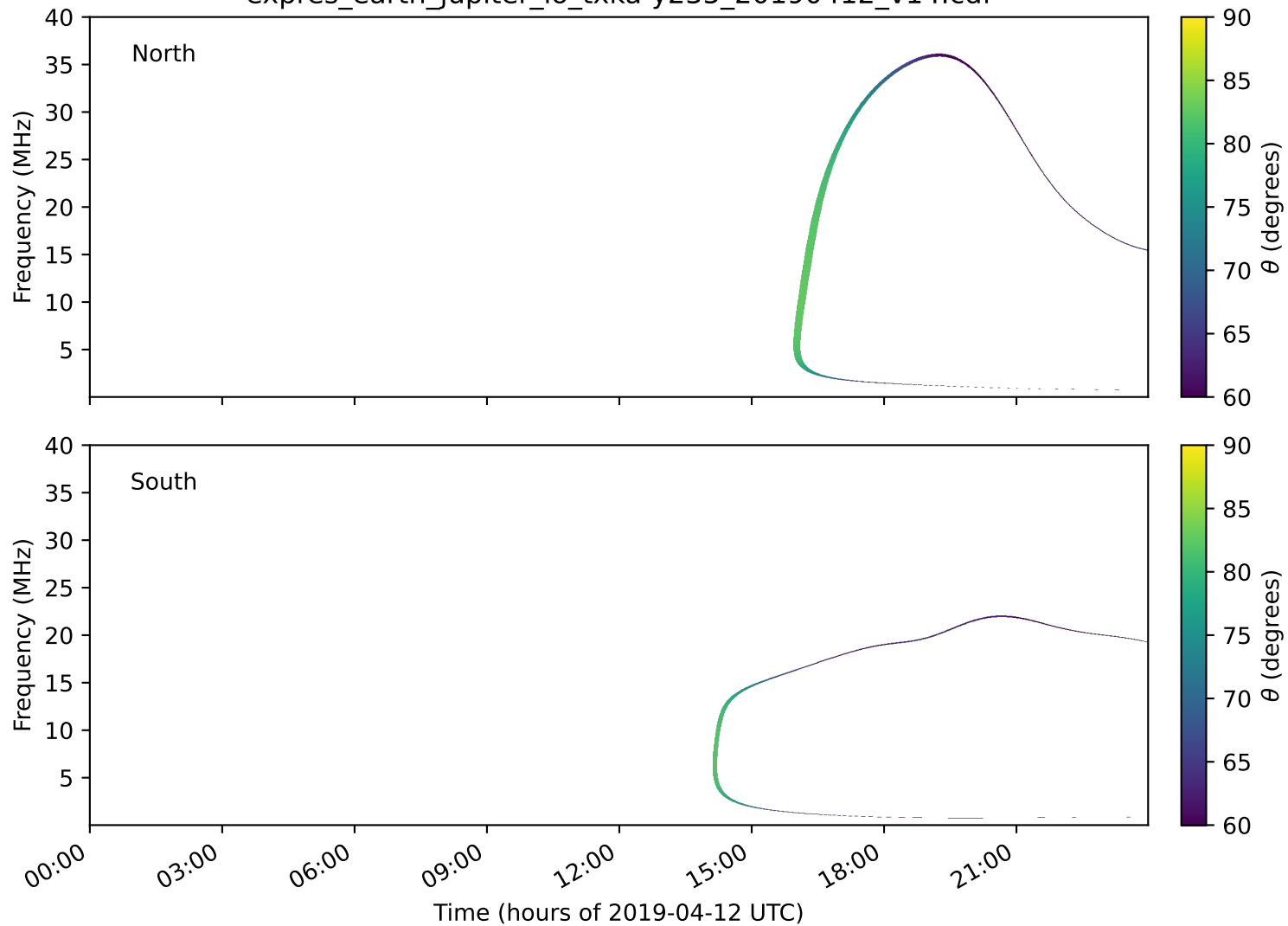
expres_earth_jupiter_io_txka-y235_20190412_v14.cdf
